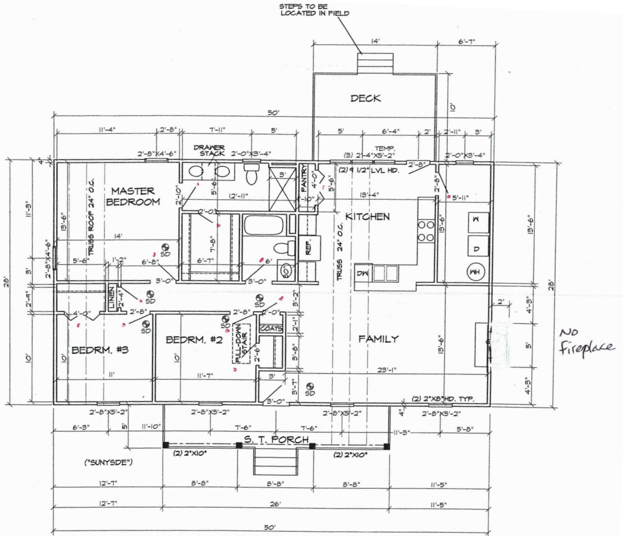
FLOOR PLAN
